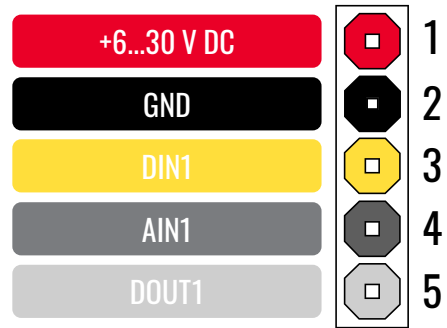
FMB910 pinout
