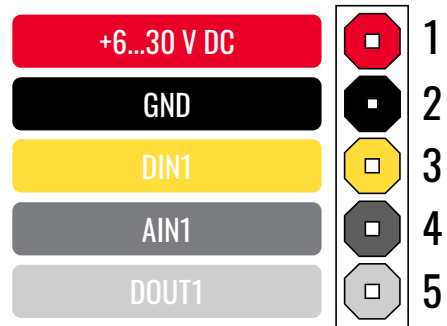
FMB900 pinout
